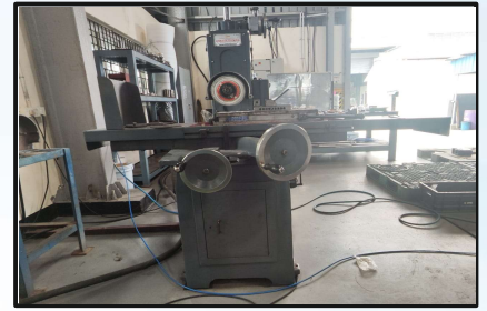
Precision Surface Grinding Machine 450x225mm
