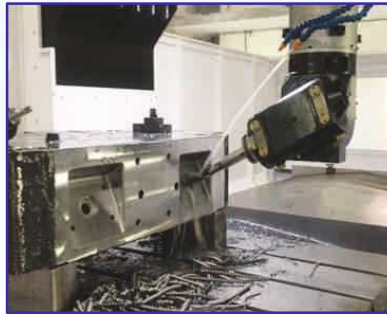
ANGULAR HEAD MACHINING
